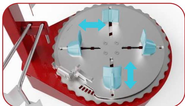
Self-centering clamp
